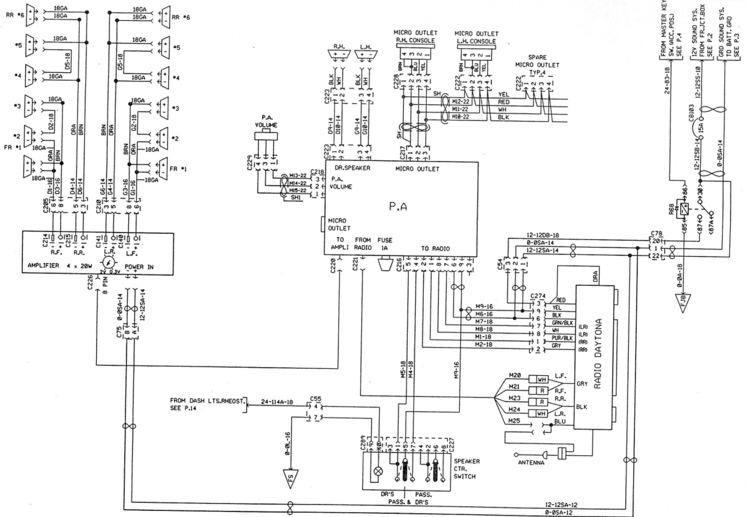
SOUND SYSTEM
