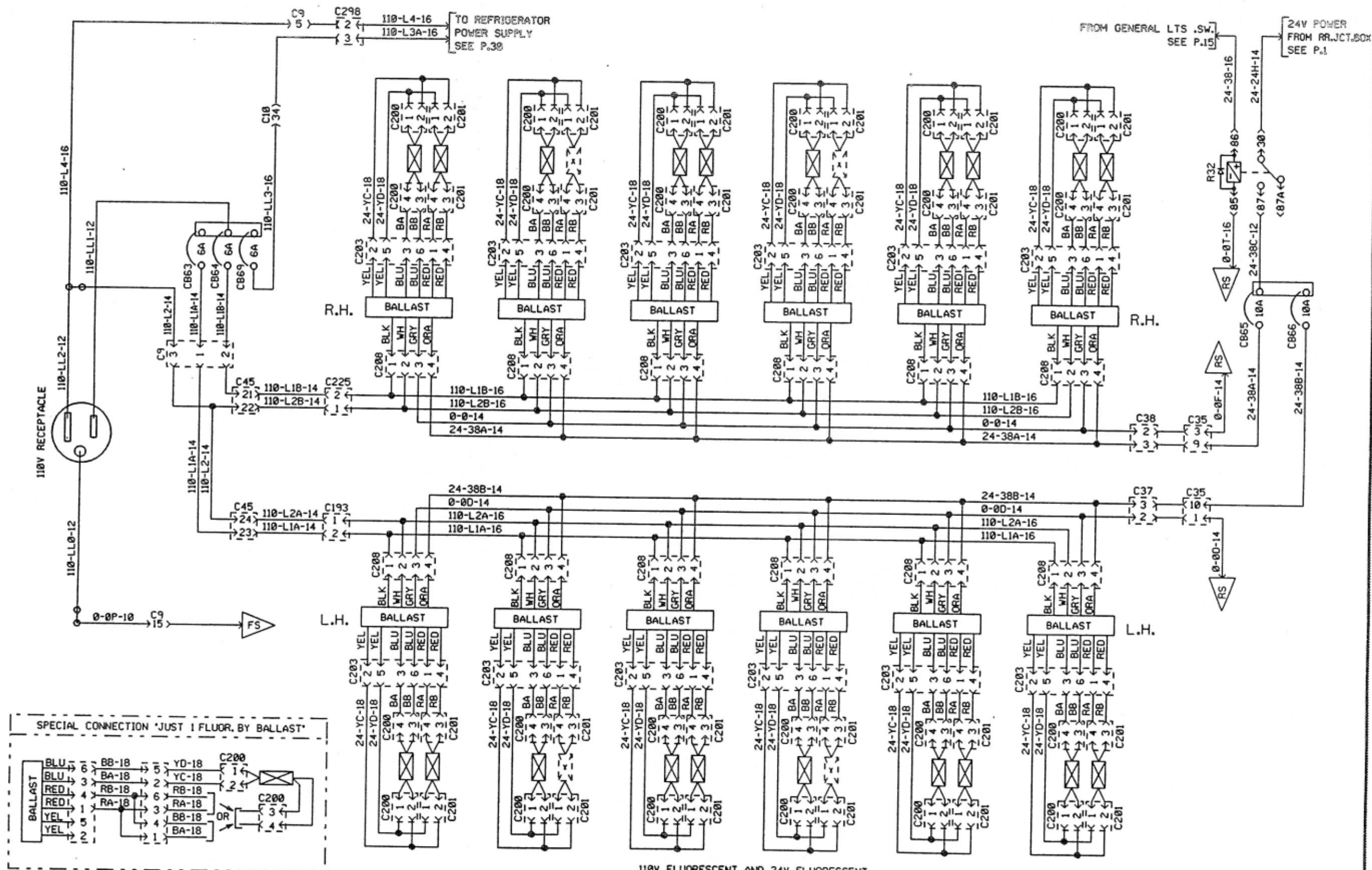
INTERIOR LIGHTING
