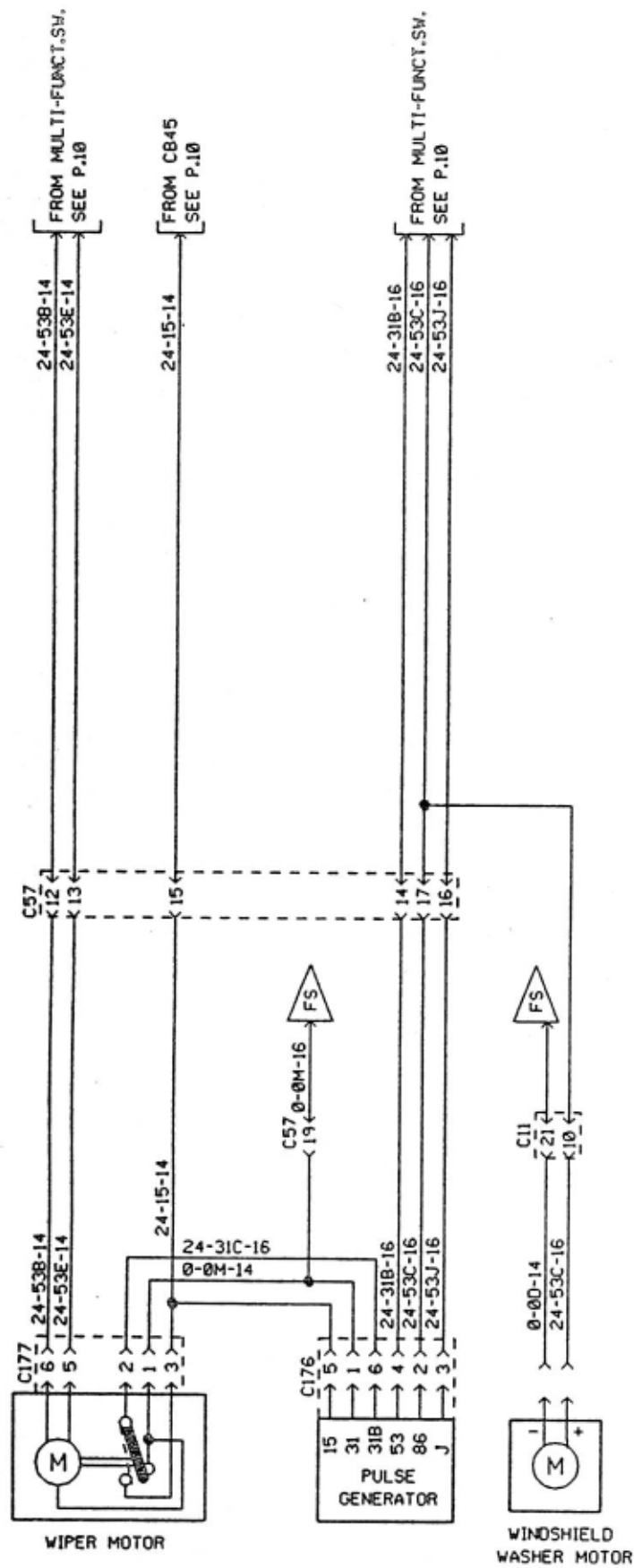
LOWER WINDSHIELD WIPER AND WASHER
